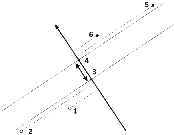
Fig. 1 Illustration of a total order that maximizes the thinnest margin between two classes. The bold double arrow stresses the margin. The bold simple arrow represents the selected vector, on which items are projected in order to form a ranking. The numbers indicate the order found
