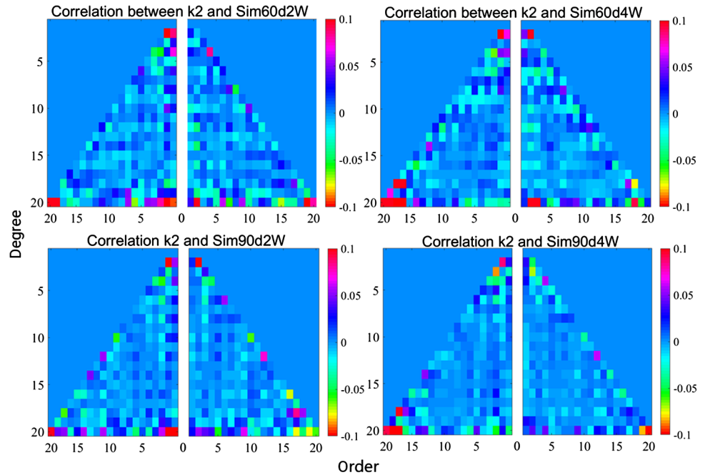
Fig. 12 Correlation between k_2 and various gravity field models. For each plot the left part is correlation between the k_2 and Cnm coefficients, and the right part is correlation between the k_2 and Snm coefficients
